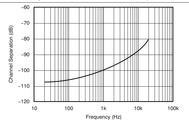
Figure 36. Channel Separation vs Frequency
