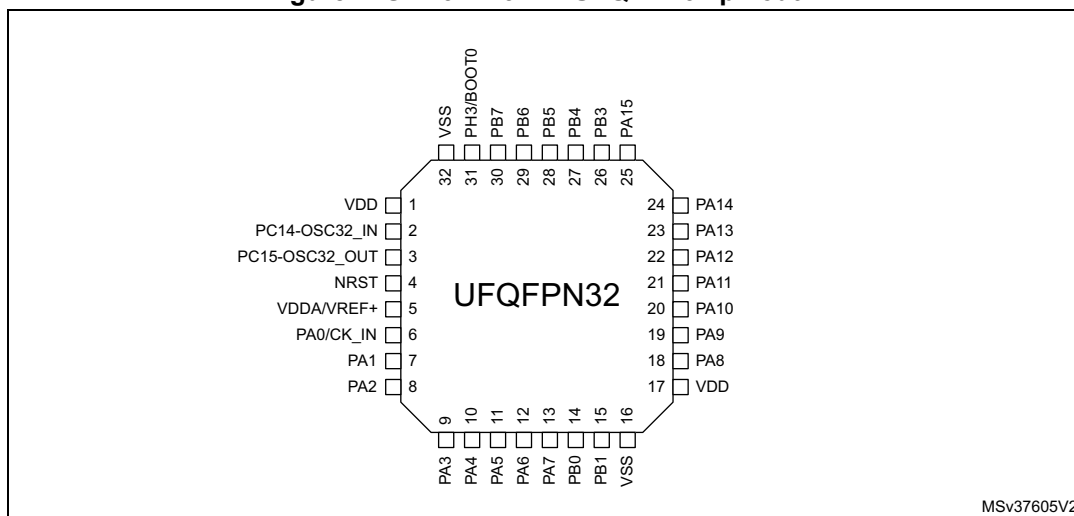
Figure 4. STM32L432Kx UFQFPN32 pinout (1)
